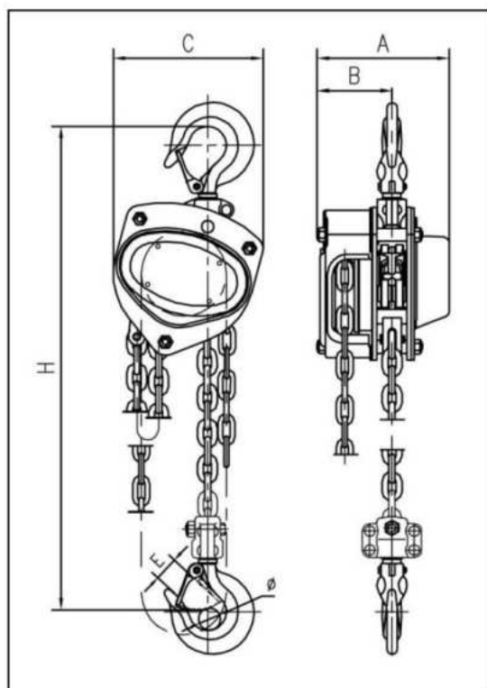
Fig. 1 Dimensioned sketch
